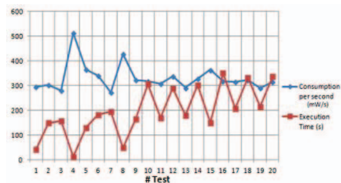
Fig. 3: Consumption per second versus Execution time per test case.
